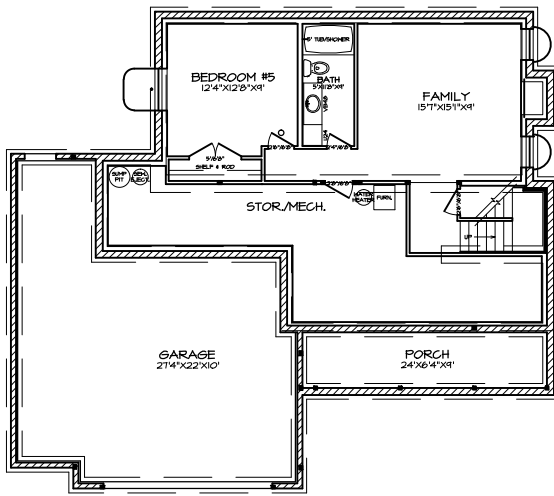
1 FOUNDATION PLAN A-3
