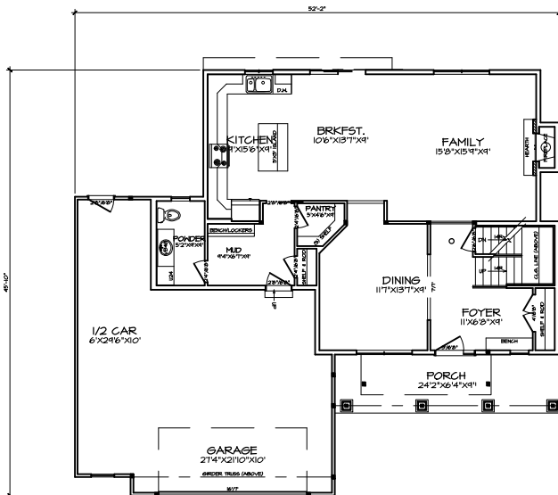
2 FIRST FLOOR PLAN A-5
