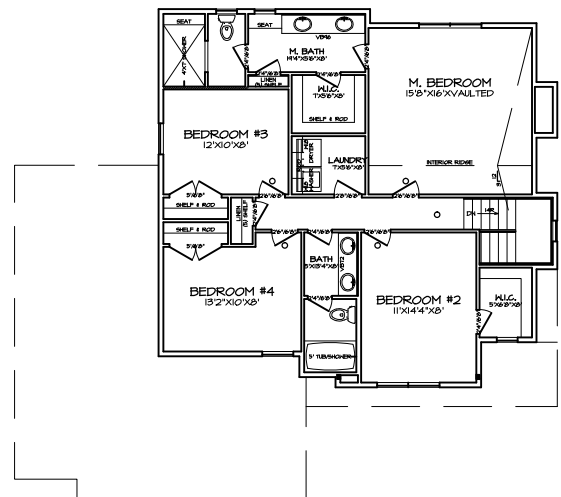
3 SECOND FLOOR PLAN A-4
